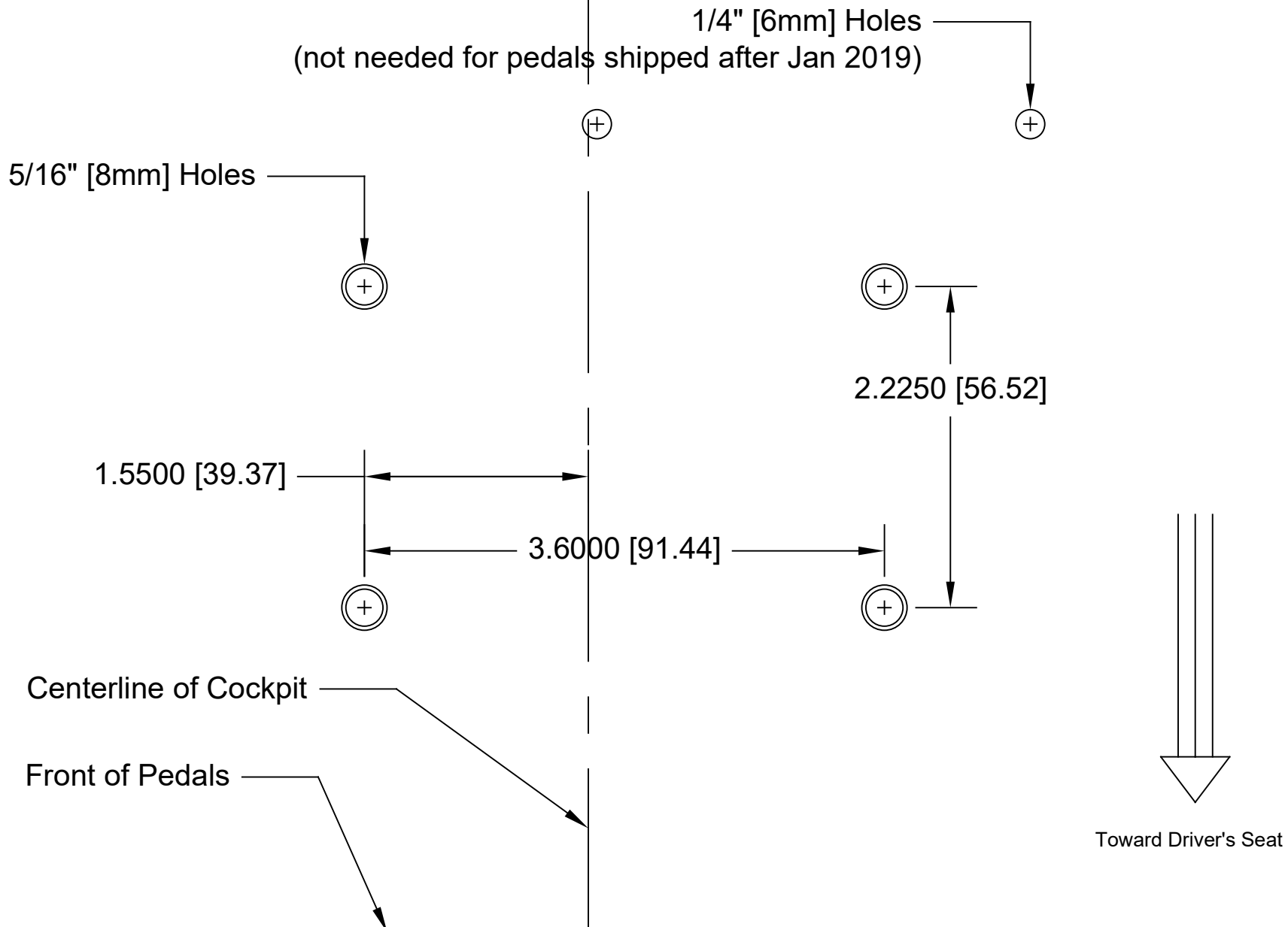
Drilling Template for Ricmotech RealGear GTpro3 Pedals
